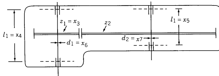
Figure 7.24 Speed reducer (gear pair) [7.40].
