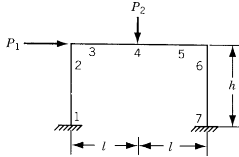
Figure 3.1 Rigid frame.
