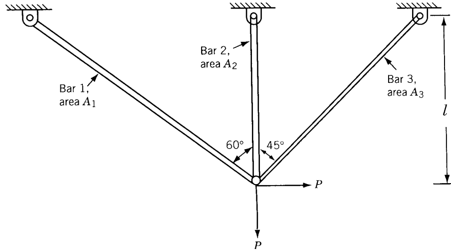
Figure 10.11 Three-bar truss.
