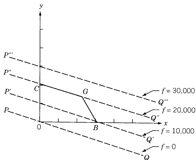
Figure 3.5 Infinite solutions.
