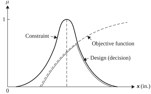
Figure 13.8 Concept of fuzzy decision. [13.22], with permission of ASME.
