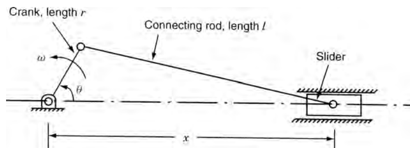
Figure 1.17 Slider-crank mechanism.
